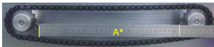
Installation and final dimensions for the ROLL-RING chain tensioner/series ISO B:
